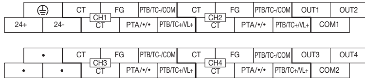
FX3U-4LC
