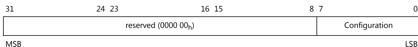
Object 1F80 h – bit structure of the value
