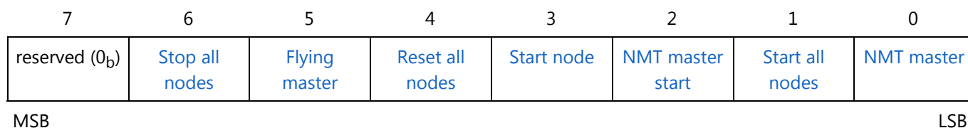
Object 1F80 h – bit structure of the configuration value
